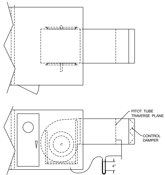
Figure 20. Air Handling Unit With Added Duct
