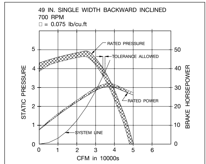
Figure 15. Field Test vs. Catalog Performance
