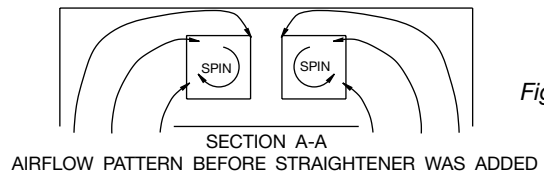
Figure 18. Duct System
