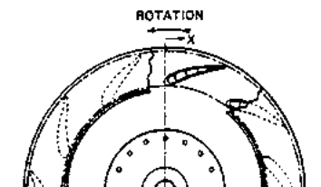
6c. Curved Airfoil, BIA
