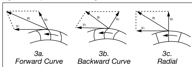
Figure 3. Impeller Vector Diagrams
