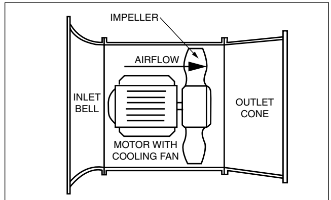
Figure 9. Direct Drive Tubeaxial Fan
