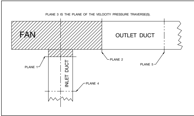
Figure 2. Measurement Reference Planes
