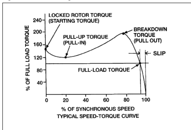
Figure 1. Motor Designs
